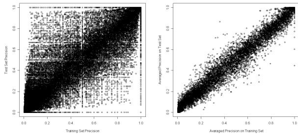
Figure 2: Precision on training set vs. precision on test set. The left graph shows the raw data (one point for each rule), while the right graphs shows the plot for averages (one point for each set of rules that cover the same number of positive and negative examples).
